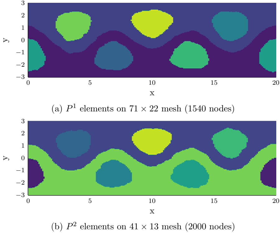
Figure 7: Bickley jet: Comparison of TO method with P^1 and P^2 elements.
