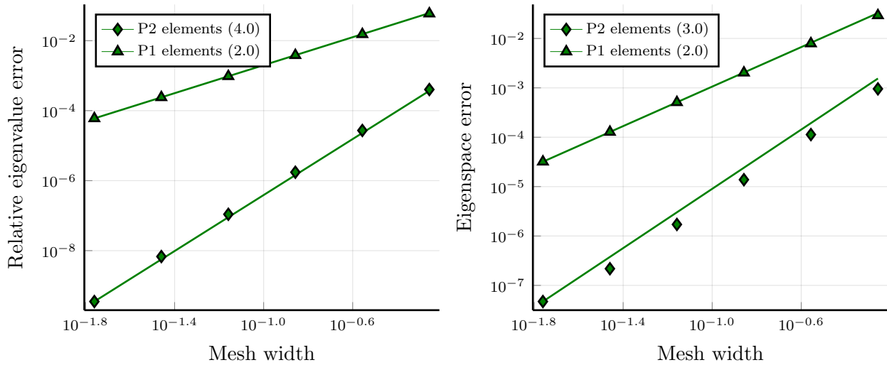
Figure 1: Standard map: Errors in the first nontrivial eigenvalue (left) and 2-dimensional eigenspace corresponding to the two smallest nontrivial eigenvalues (right) of the dynamic Laplacian with the CG approach. The slopes of the corresponding lines are given in brackets in the legends.
