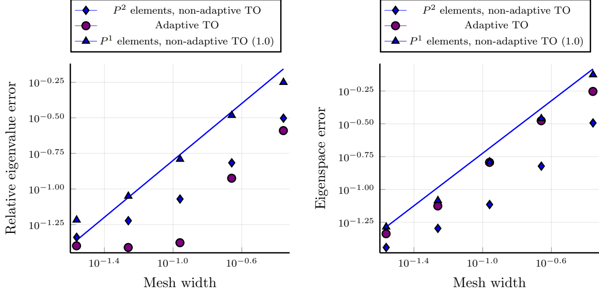
Figure 6: Cylinder flow: Errors in the first nontrivial eigenvalue (left) and corresponding eigenspace (right) of the dynamic Laplacian for the TO approaches. The slopes of the corresponding lines are given in brackets in the legends.
