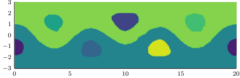
(b) P^2 elements on 21 \times 7 mesh (720 quadrature points, 240 triangles)
