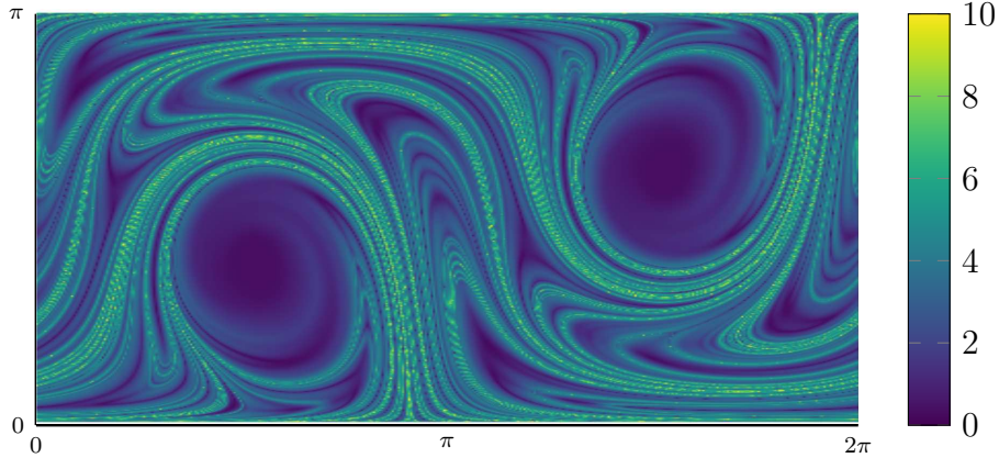
Figure 3: Cylinder flow: log of the trace of the mean diffusion tensor, \log_{10} \text{tr}(A(x)) .
