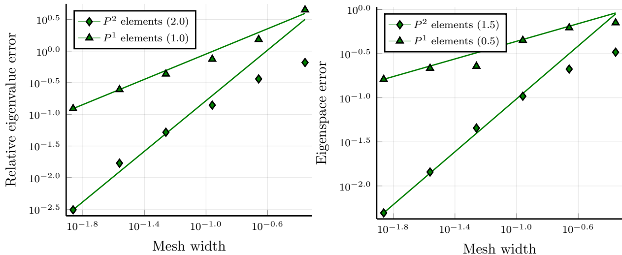
Figure 2: Cylinder flow: Errors in the first nontrivial eigenvalue (left) and corresponding 1-dimensional eigenspace (right) of the dynamic Laplacian discretized with CG approach. The slopes of the corresponding lines are given in brackets in the legends.
