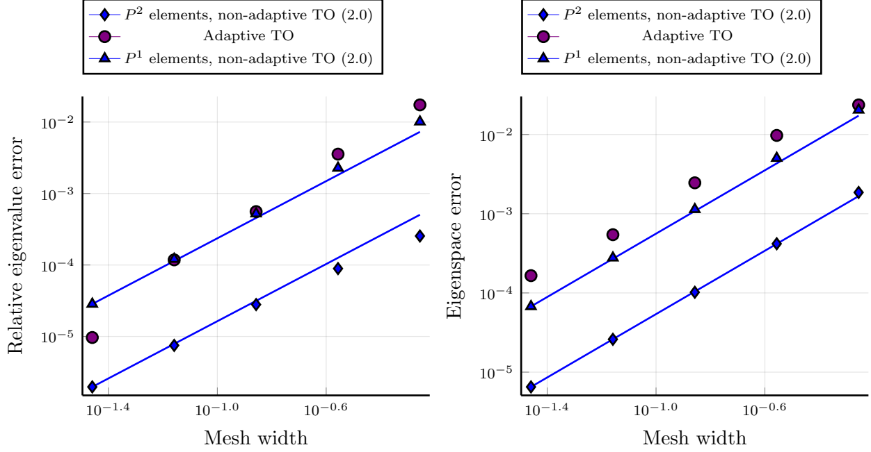
Figure 5: Standard map: Errors in the first nontrivial eigenvalue (left) and 2-dimensional eigenspace spanned by the smallest eigenvectors (right) of the dynamic Laplacian discretized with the TO approach. The slopes of the corresponding lines are given in brackets in the legends.
