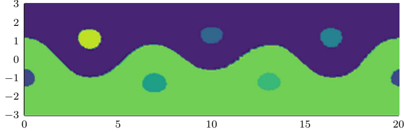
(a) P^1 elements on 101 \times 31 mesh (18000 quadrature points, 6000 triangles)
