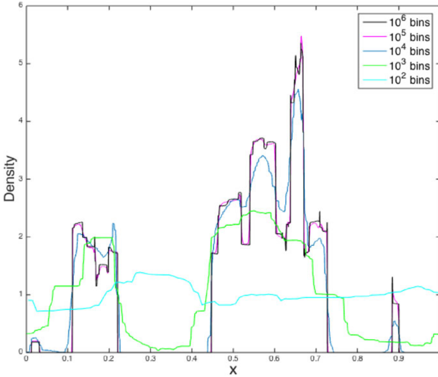
FIGURE 2. Approximations to the density of the quenched random measure \mu_\omega|_{\omega=0.4260} , computed via Ulam’s method at differing levels of accuracy.
