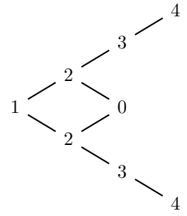
F(D_5, 4)
