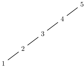
F(A_5, 1)
