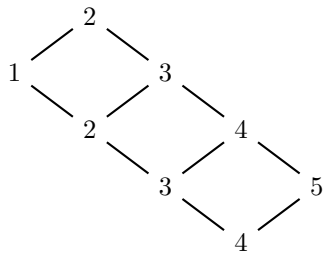
F(A_5, 4)
