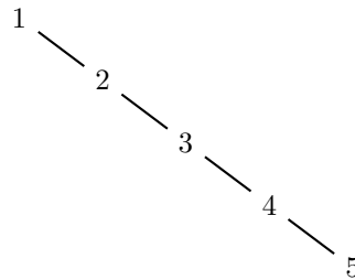
F(A_5, 5)
