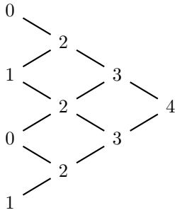
F(D_5, 1)
