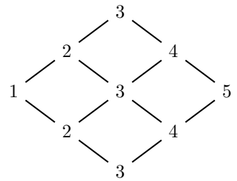
F(A_5, 3)
