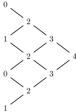
F(D_5, 1)
