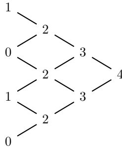
F(D_5, 0)
