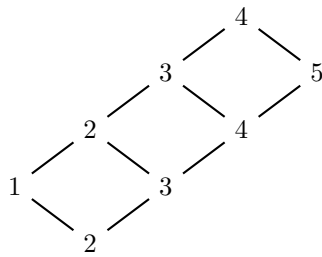
F(A_5, 2)
