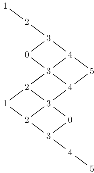
F(E_6, 5)
